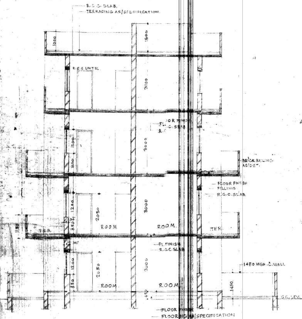
SECTION E-3
